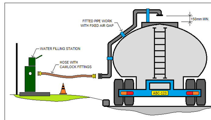
Option A – Fitted pipe work with fixed air gap (Preferred)
