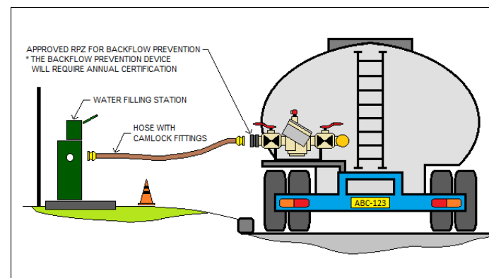
Option B – Bottom fill via approved RPZ
