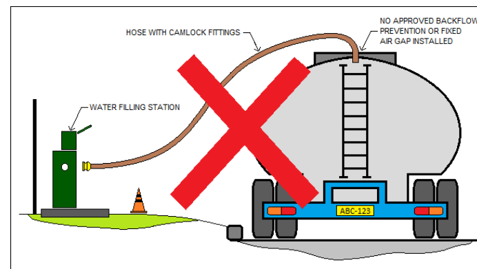
Top fill (Not Approved)
