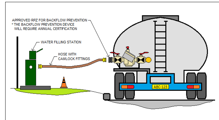
Option B – Bottom fill via approved RPZ
