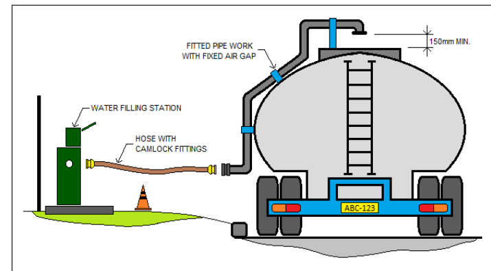
Option A – Fitted pipe work with fixed air gap (Preferred)
